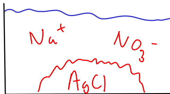
Insoluble \text{AgCl} falls out of solution as it is formed - "precipitation"
