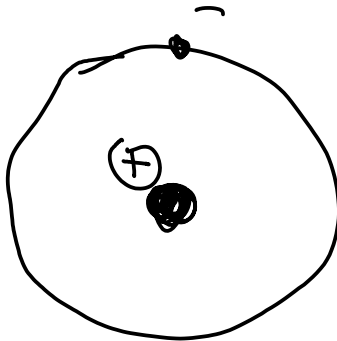
Hydrogen-2 "Deuterium"
