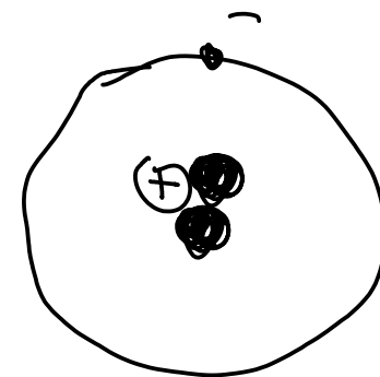
Hydrogen-3 "Tritium"
